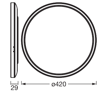
PANEL ESSENTIAL 420 28W 840 WT
