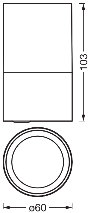
ENDURA CLA TUBE DOWN C GU10 IP54 DG
